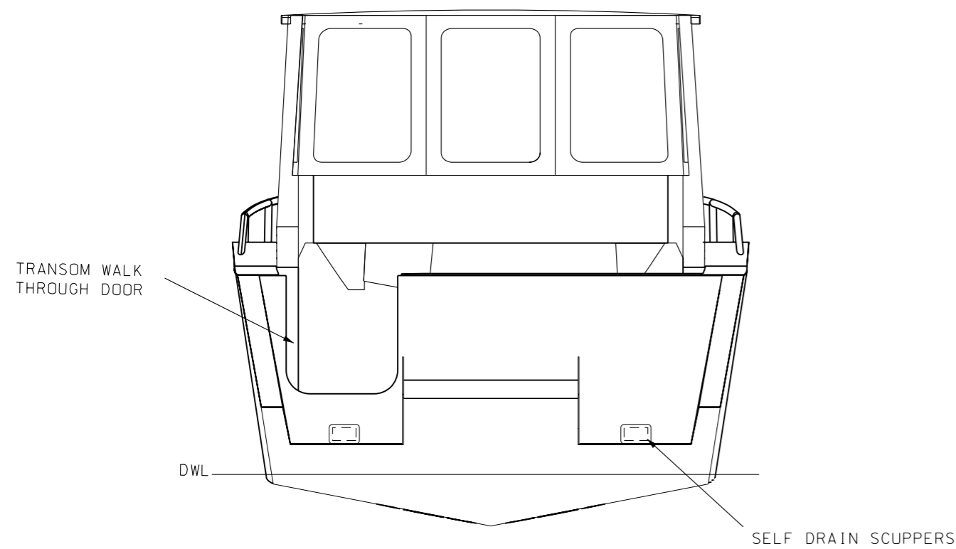
REAR BODY
