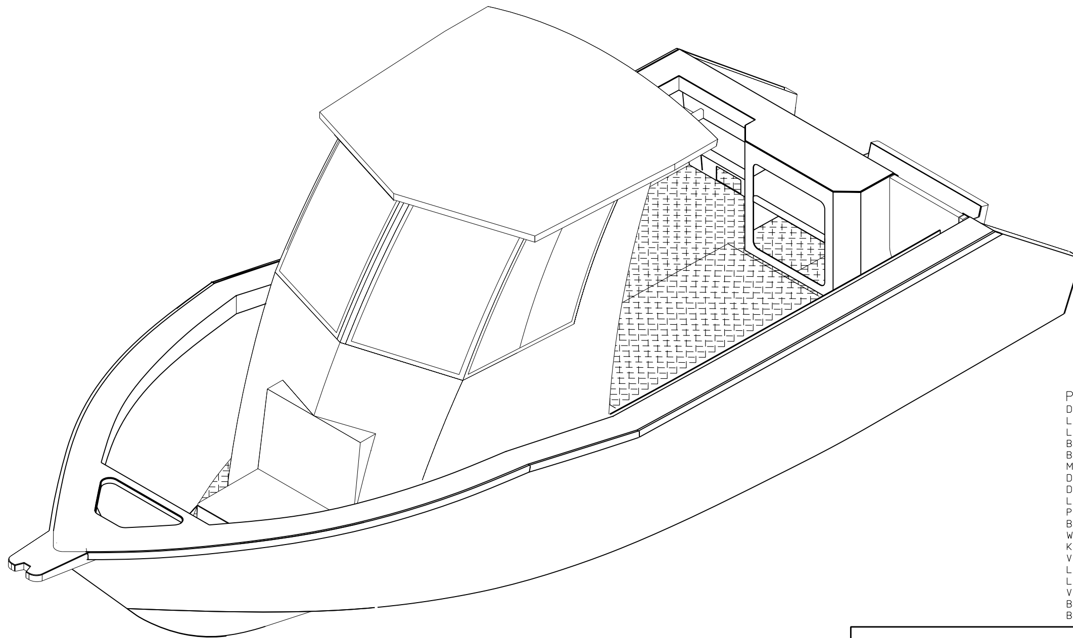
ISOMETRIC VIEW
